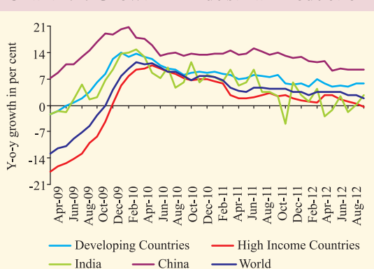
Chart I.2: Growth in Industrial Production
