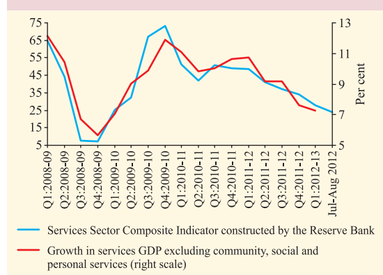
Chart I.11: Services Sector Composite Indicator
