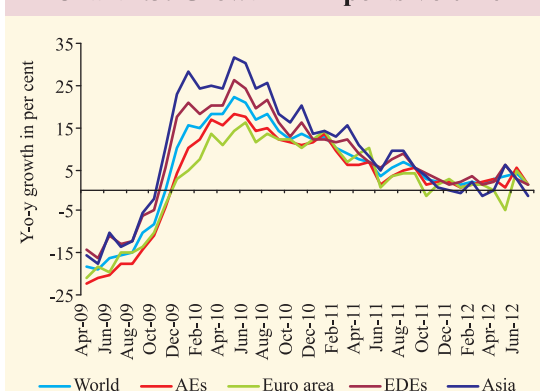
Chart I.3: Growth in Exports Volume
