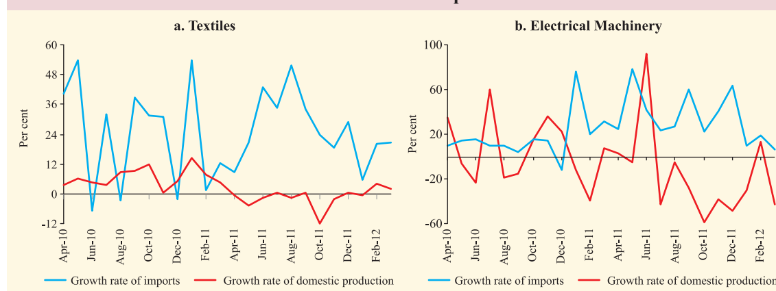
Chart I.8: Domestic Production vis-à-vis Imports of Manufactured Goods
