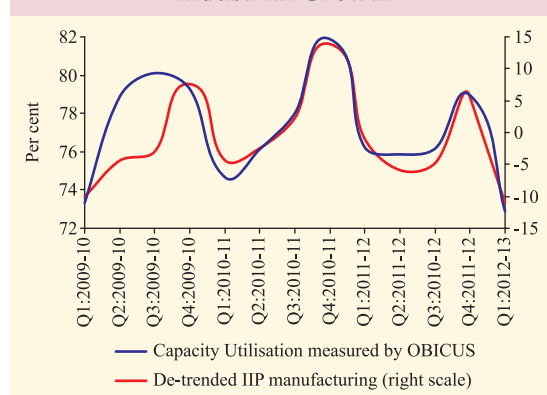
Chart I.10: Capacity Utilisation and Industrial Growth
