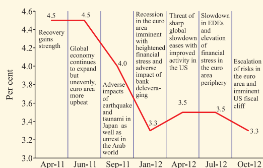
Chart I.1: IMF Projections for Global Growth in 2012
