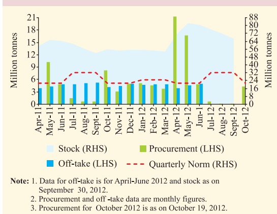
Chart I.6: Food Stock and its Determinants
