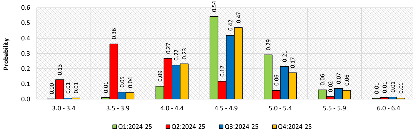
Chart 2: Probability distribution of CPI inflation forecast from Q1:2024-25 to Q4:2024-25
