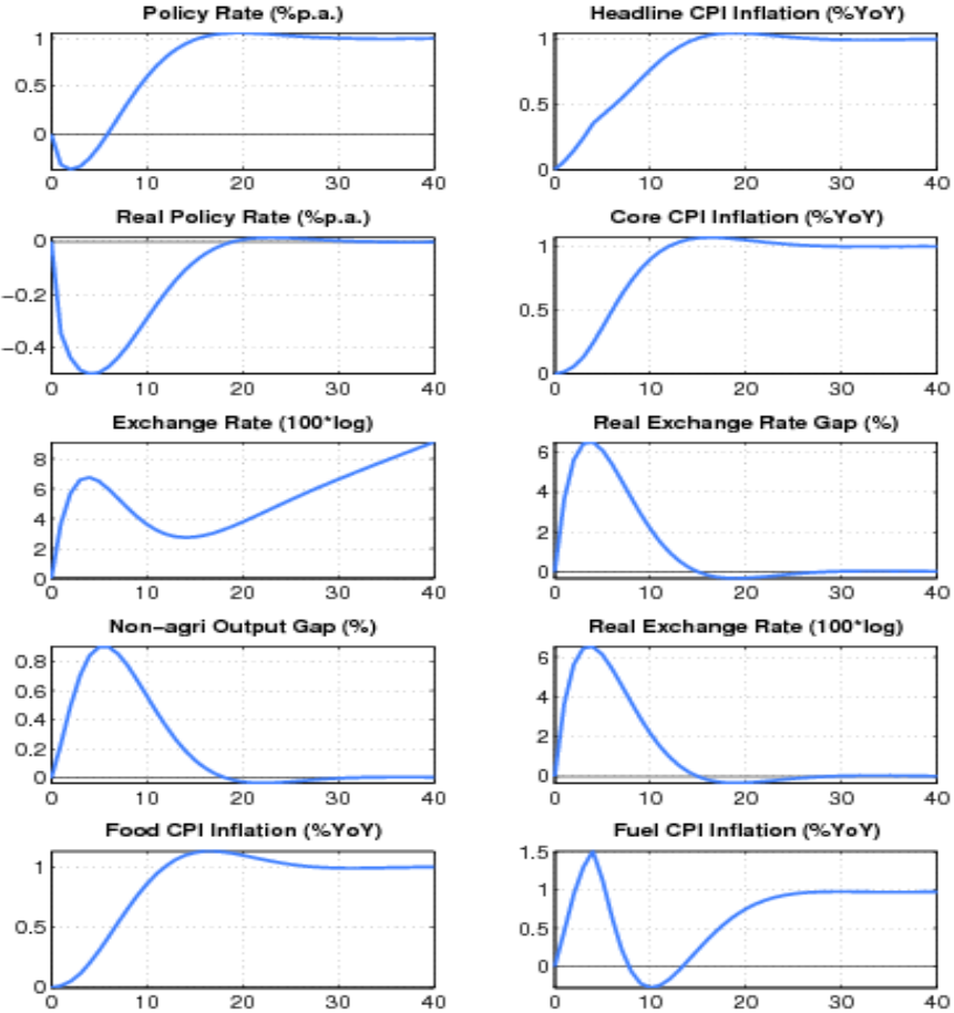
Figure 3. Response to a 1Percentage Point Increase in the Inflation Target – Imperfect Credibility
