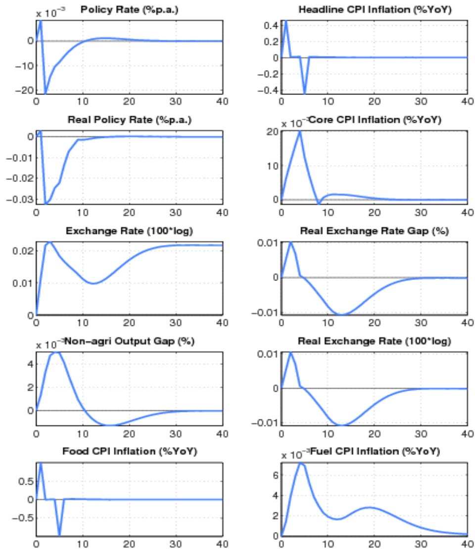
Figure 9. Response to a 4 Percentage Point Increase in Food Inflation (Annualized QoQ) due to Vegetable Price shock
