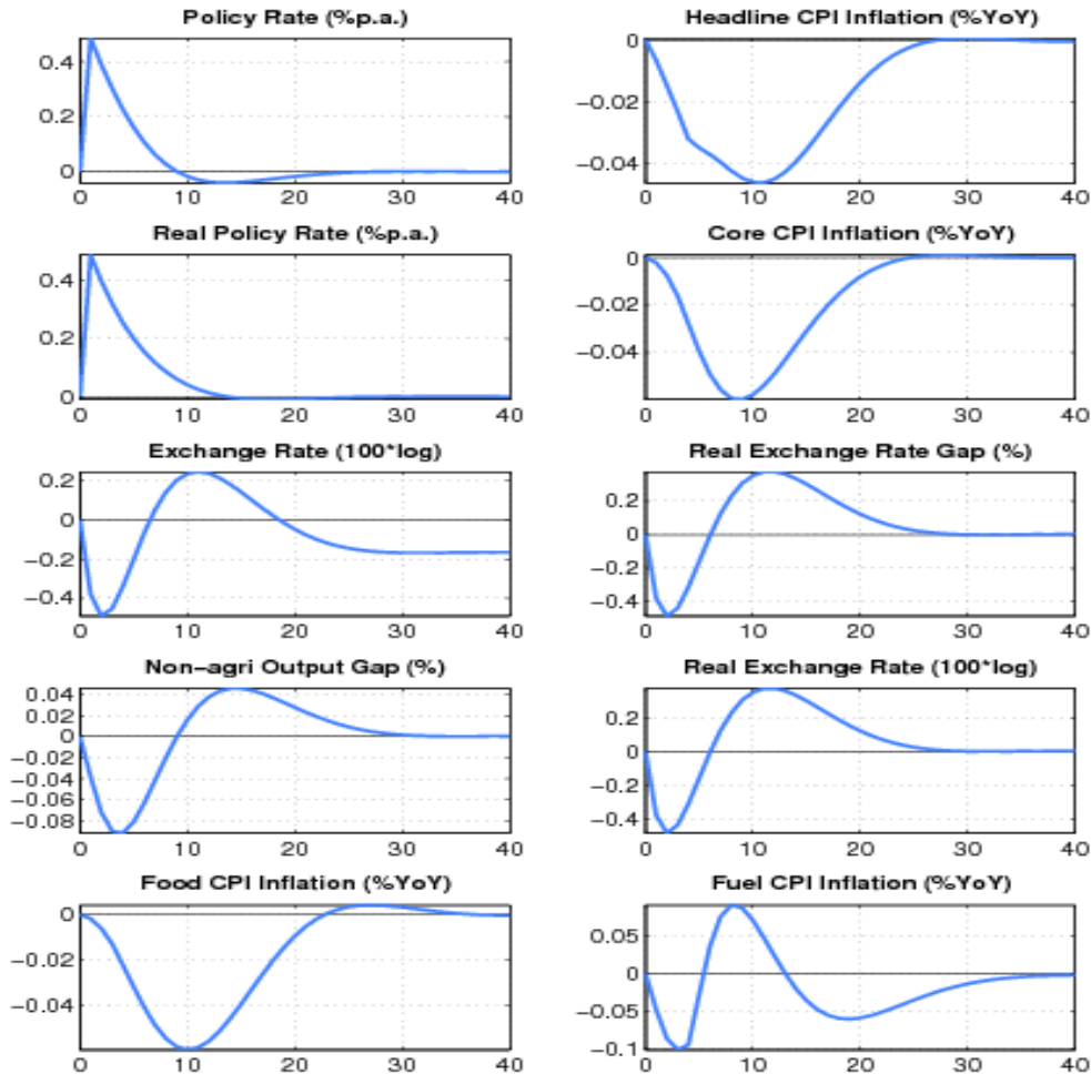
Figure 4. Response to a 0.5 Percentage Point Increase in the Policy Rate
