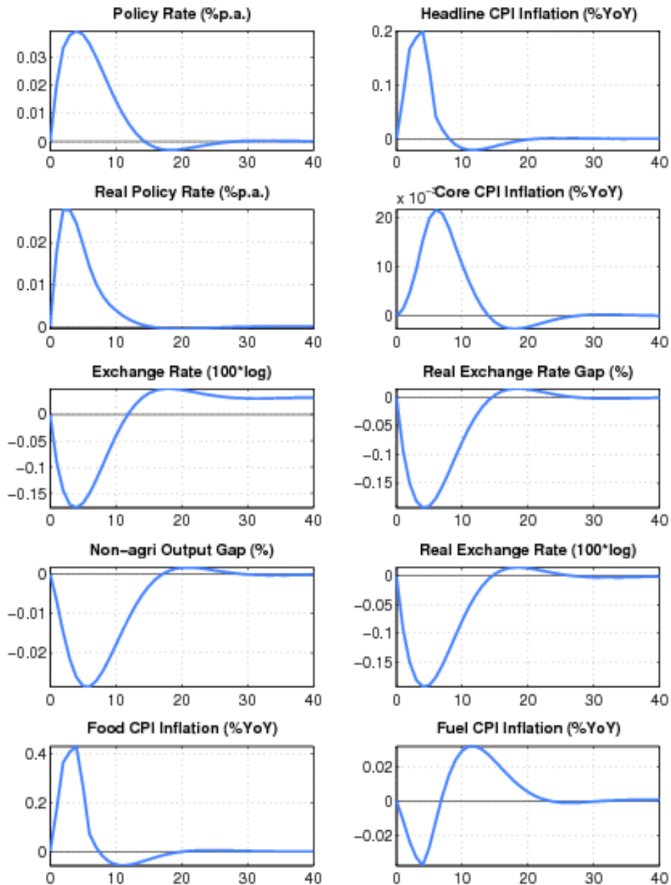
Figure 8. Response to a 1 Percentage Point Increase in Food Inflation (Annualized QoQ) due to MSP shock
