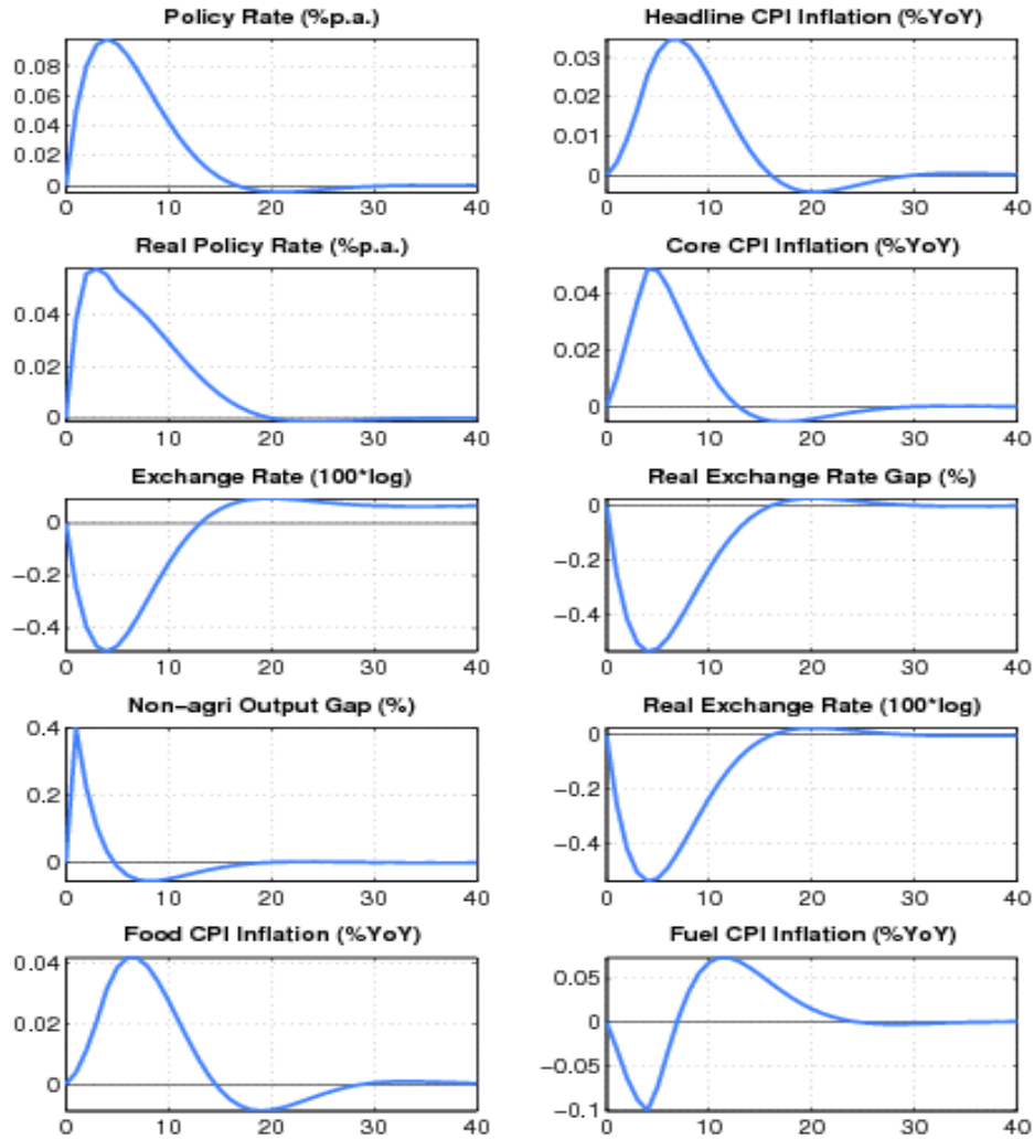
Figure 5. Response to a 0.4 Percentage Point Increase in the Output Gap
