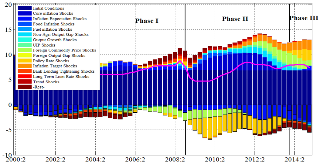
Figure 11. Historical Shock Decomposition for the Policy Rate
