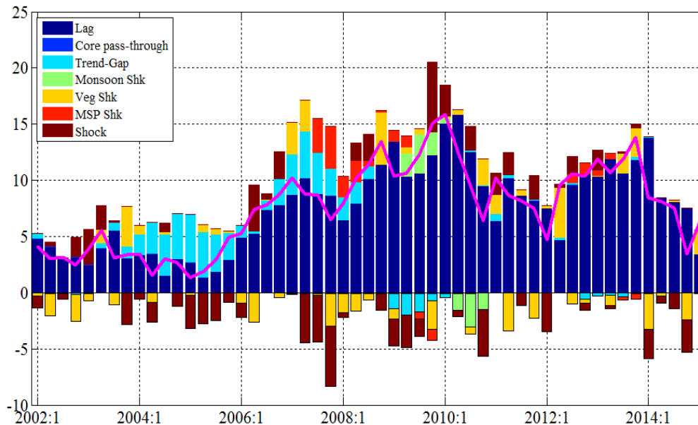
Figure 13. Historical Variable Decomposition for Food Inflation
