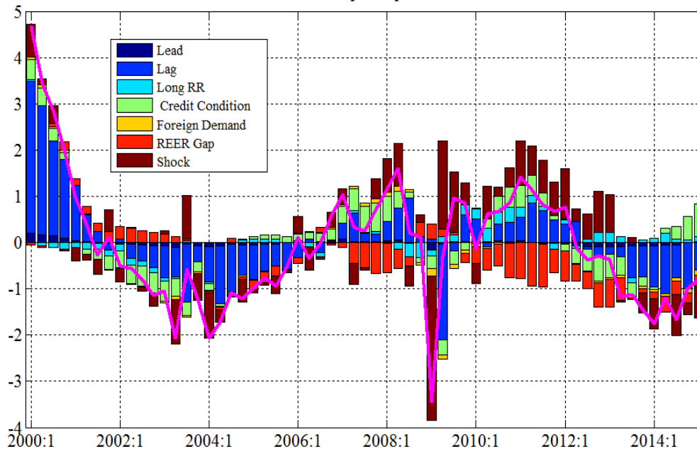
Figure 12. Historical Variable Decomposition for Output Gap
