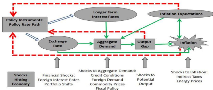
Box Figure 1. Monetary Policy Model: IFT Feedback Response and Transmission
