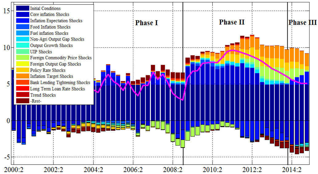
Figure 10. Historical Shock Decomposition for Core Inflation
