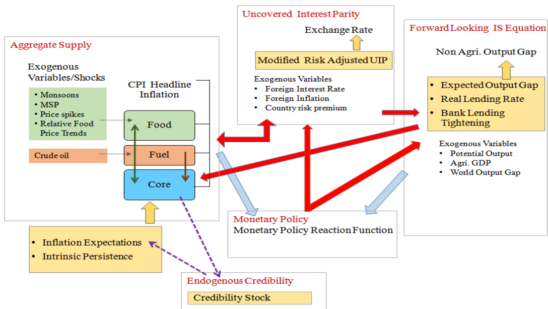
Figure 2: Production QPM: Key Blocks and Transmission Mechanism
