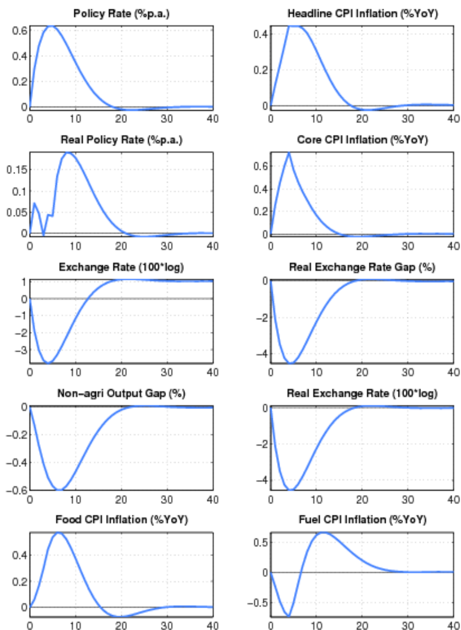
Figure 6. Response to a 1 Percentage Point Increase in Core Inflation (Annualized QoQ)
