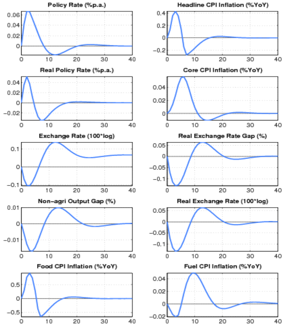
Figure 7. Response to a 2 Percentage Point Increase in Food Inflation (Annualized QoQ) due to Monsoon
