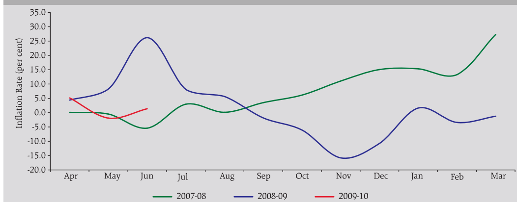
Chart 36: Annualised M-o-M seasonally adjusted inflation of WPI-All Commodities
