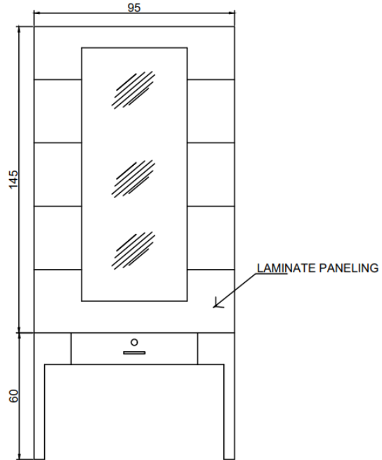
DRESSING TABLE DETAILS
