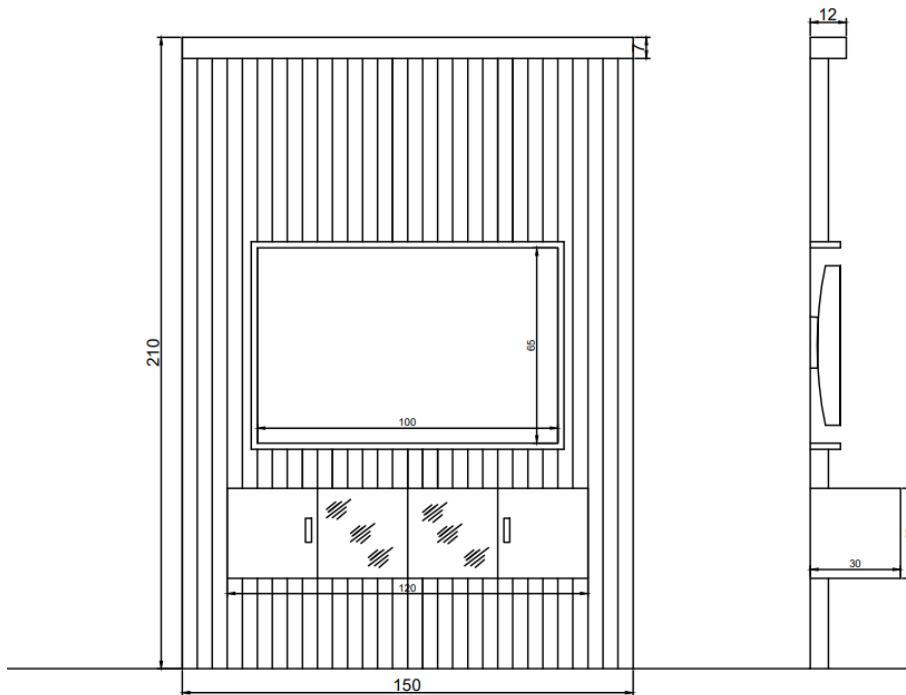
TV CABINET DETAILS
