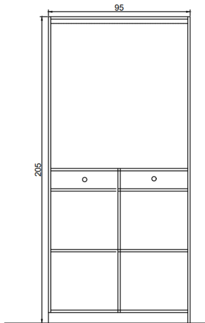
WARDROBE DETAILS
