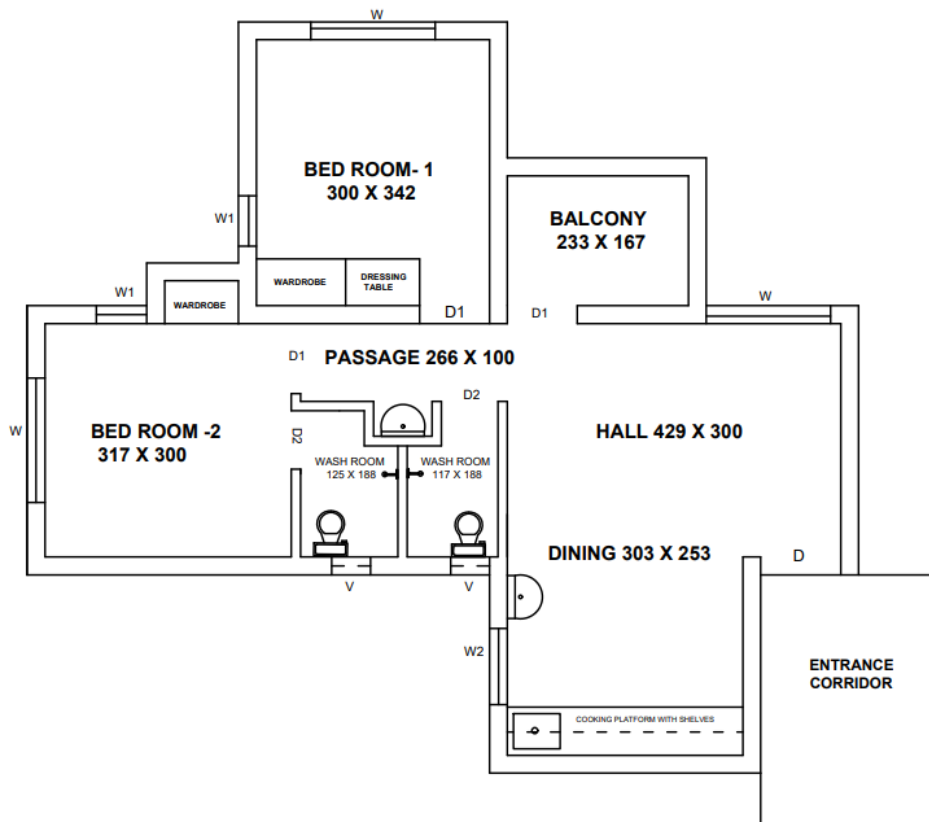
TRANSIT HOLIDAY HOME FLAT AT THAMALAM PROPOSED LAYOUT
