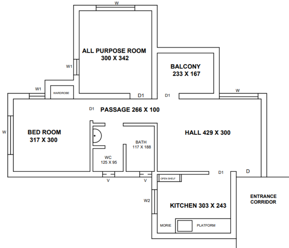
CLASS III FLAT AT THAMALAM TYPICAL LAYOUT
