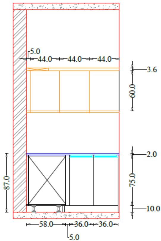
Elevation C
