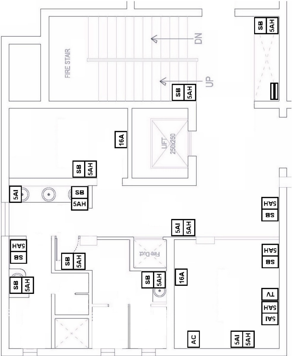
Passage Area- 3F- OB- Points
